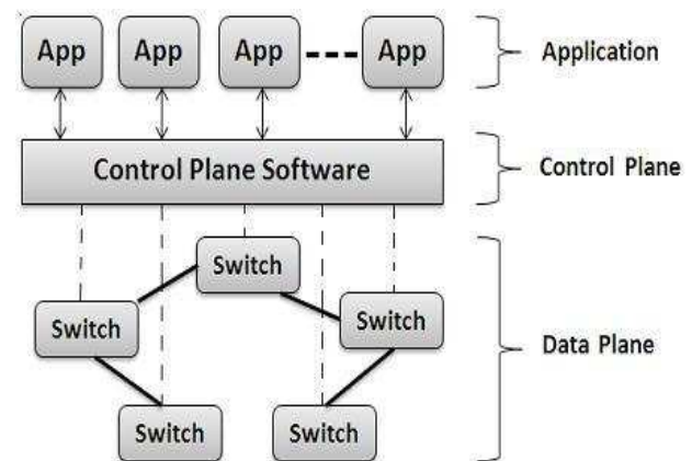
Figure 1. SDN Architecture.
