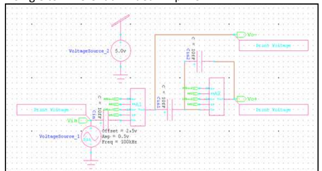
Figure 10: Design Of Single To Differential Ended Amplifier Using PFG Inverter
