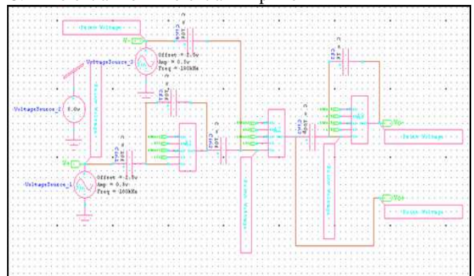
Figure 12: Design of Differential To Differential Amplifier Using PFG Inverter
