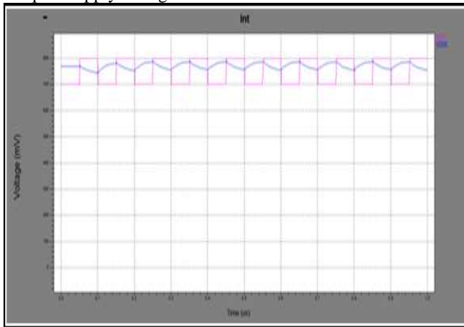
Figure 7: Response Of Integrator For Square Wave Input
