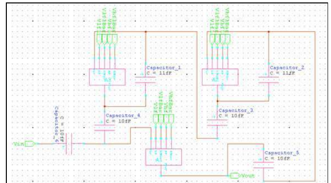
Figure4: Differentiator using PFG inverter
