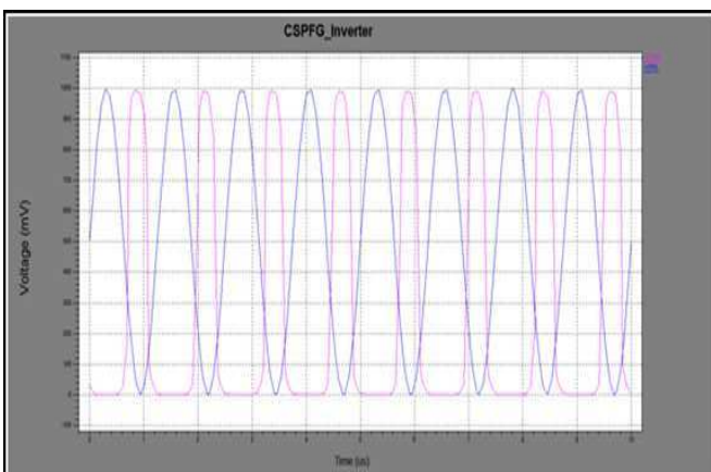
Figure3: input output waveform of inverter
