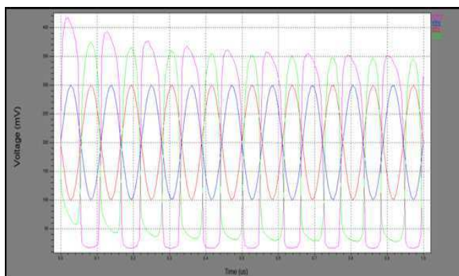
Figure 15: Response Of Differential To Differential High Gain Amplifier Using PFG Inverter
