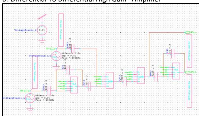
Figure 14: Design Of Differential To Differential High Gain Amplifier Using PFG Inverter
