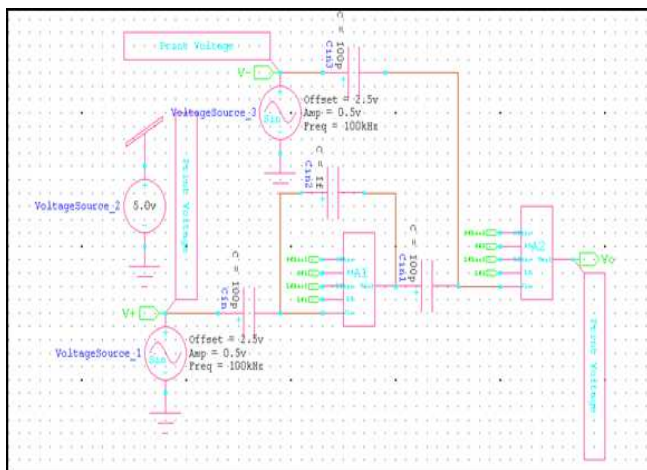
Figure 8: Design of differential to single ended amplifier Using PFG Inverter
