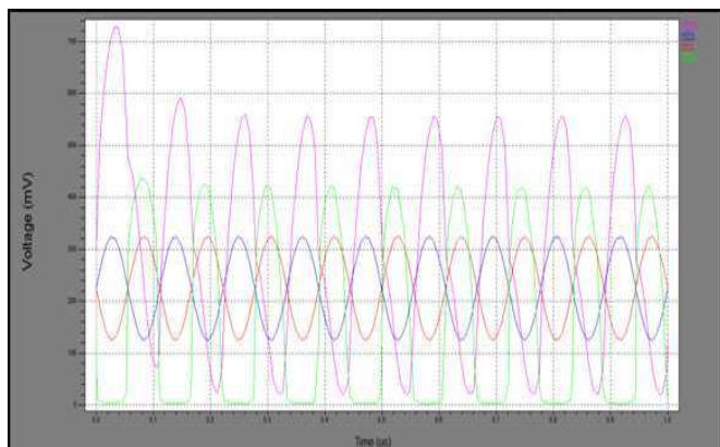
Figure 13: Response Of Differential To Differential Amplifier Using PFG Inverter
