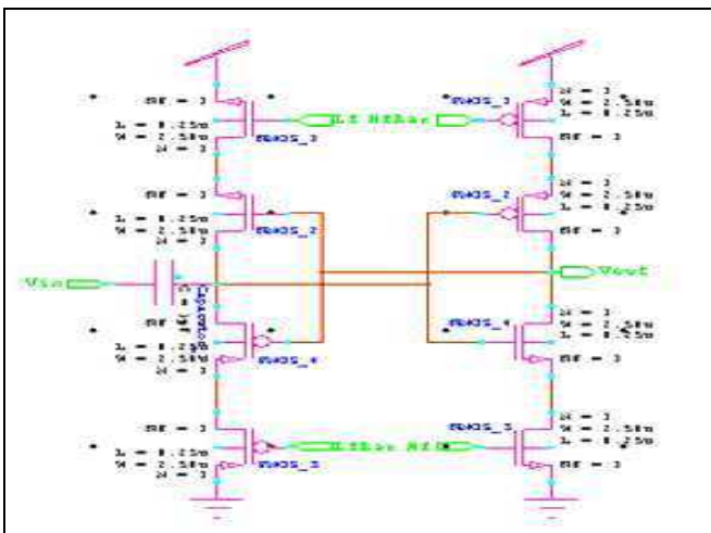
Figure2: PFG inverter
