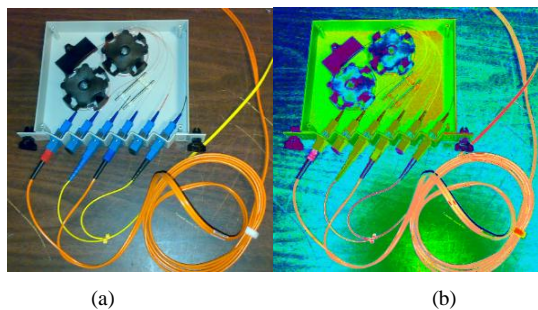
Figure 5. Visual Inspection of optical fiber cables in an optical coupler reveals the existence of electrical anomalies (Sample 1) a) RGB regular image and b) Thermal Image
