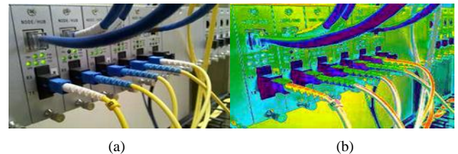
Figure 7. Visual Inspection of optical Router-Switch cables reveals the existence of electrical anomalies (Sample 3) a) RGB regular image, b) Thermal Image
