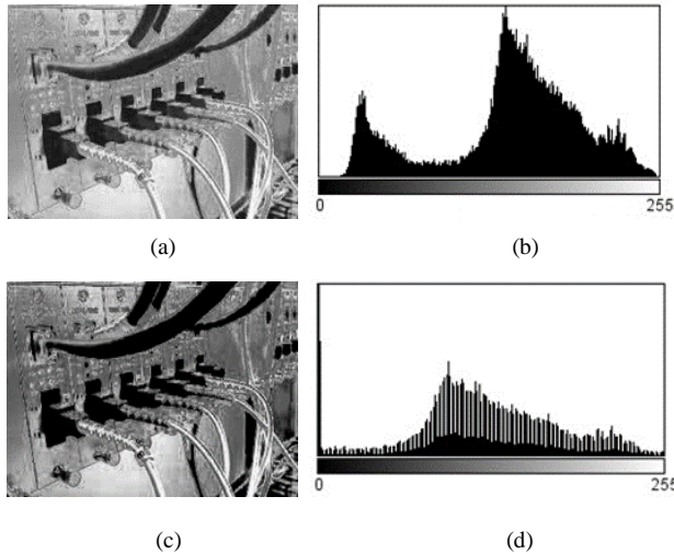
Figure 10. Sample 3: a) Gray scale of thermal image b) Histogram chart for (Gray scale of thermal image) c) Histogram Equalization for (Gray scale of thermal image) d) Histogram chart for (Histogram Equalized image)
