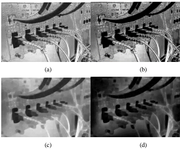
Figure 18. Sample 3: a) Thermal image Gray scale b) Resulting image after histogram equalization c) Image after morphological operation d) Restored image after the FFT transform
